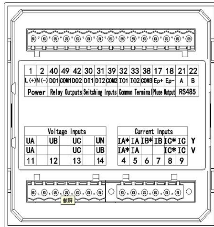
Figure 8 AMC96 series terminal block diagram
