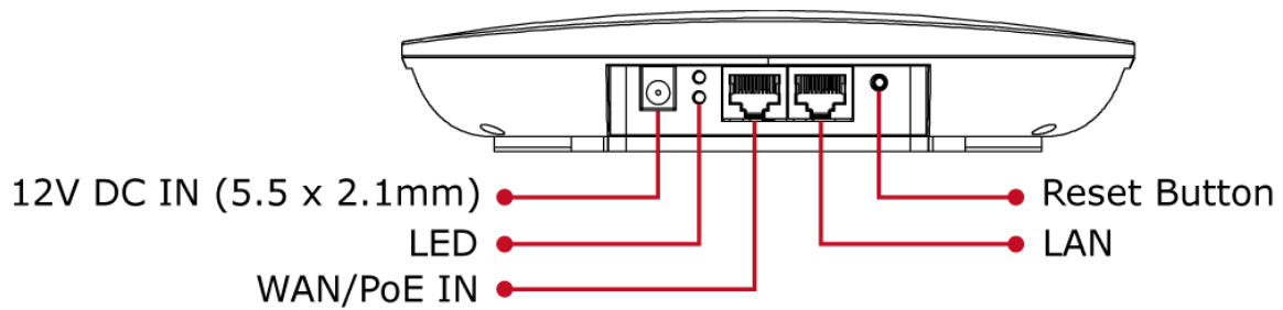
Figure 2-4 WDAP-C7210E Bottom Panel
