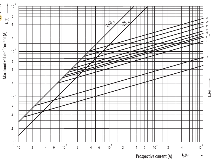
Cut-off current characteristics CH8
