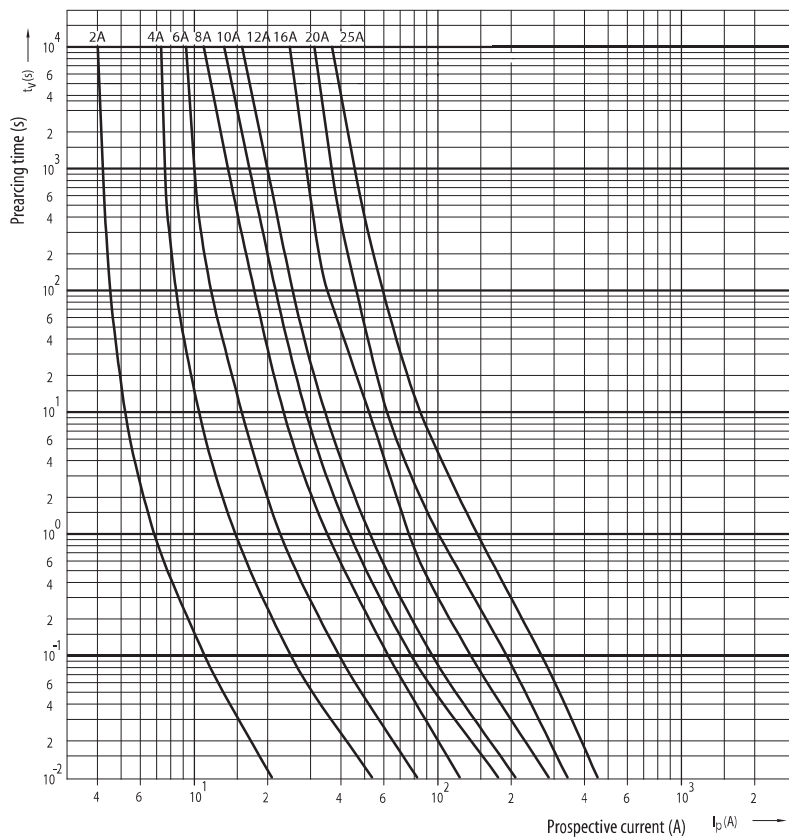
Time current characteristics I/t, gG CH8
