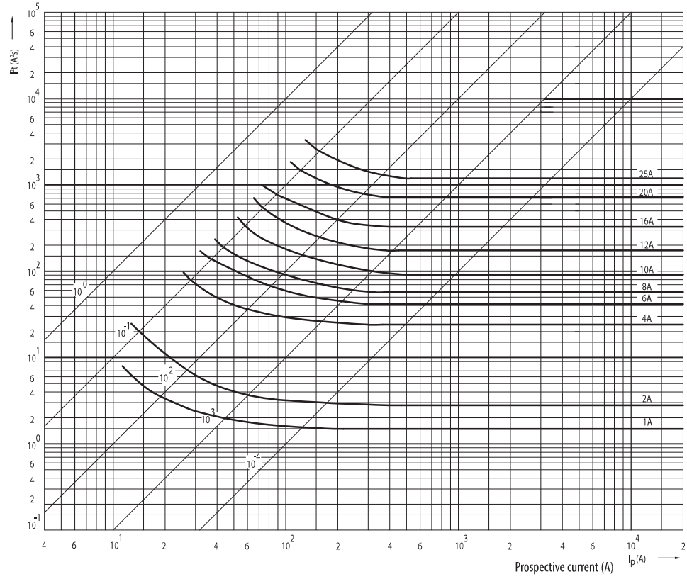
Melting energy characteristics I 2 t CH8
